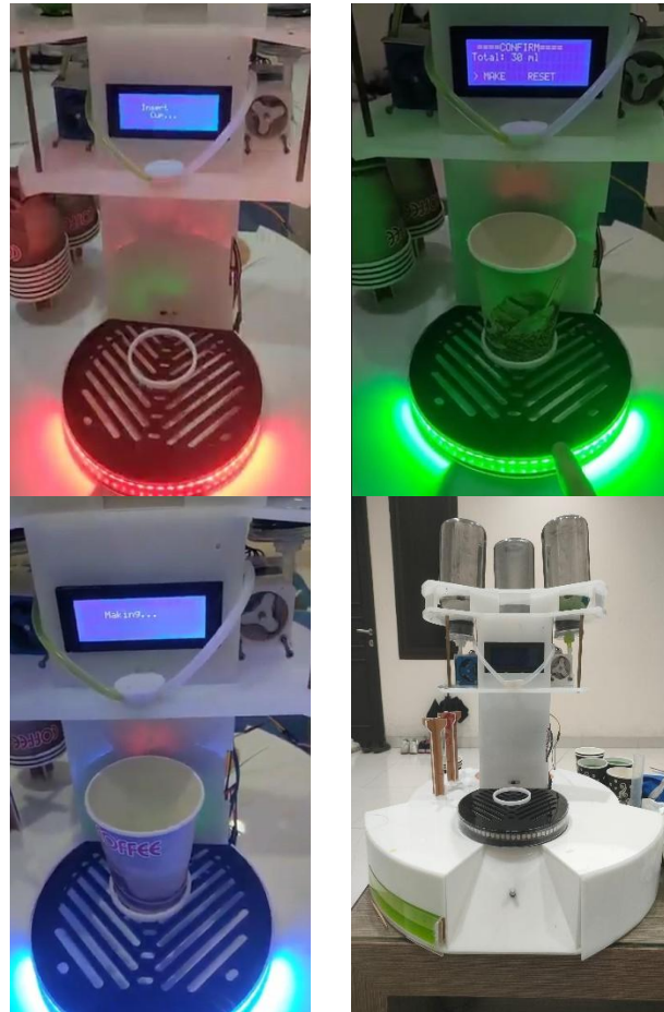
Fig. 1. Appearance of Automatic Drink Dispensing System
